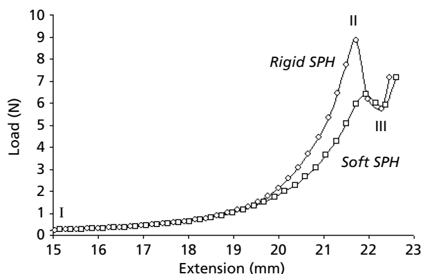
Figure 4 SPH mechanogram obtained from a regular mechanical tester.
