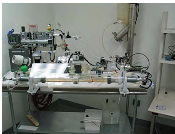
Figure 5 Gastric simulator.
